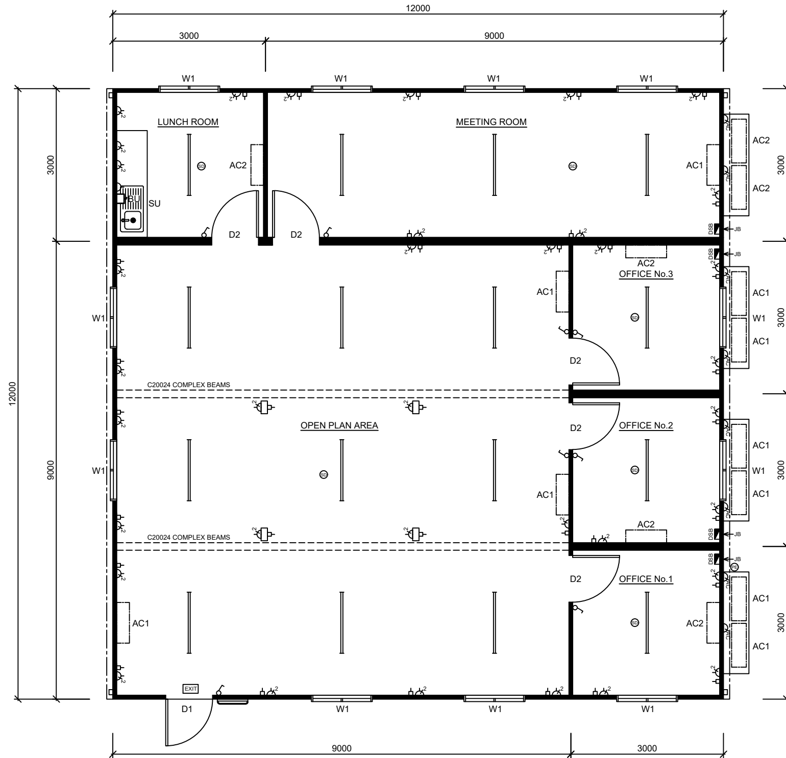
12.0x12.0m Office Complex - Floor Plan
