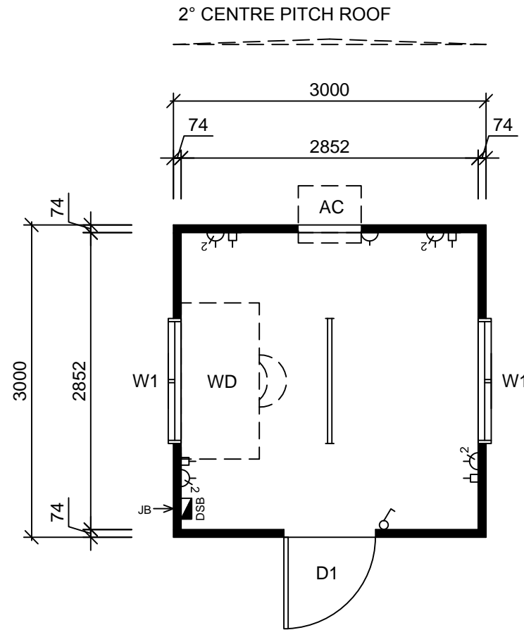
3.0x3.0m Office - Floor Plan
