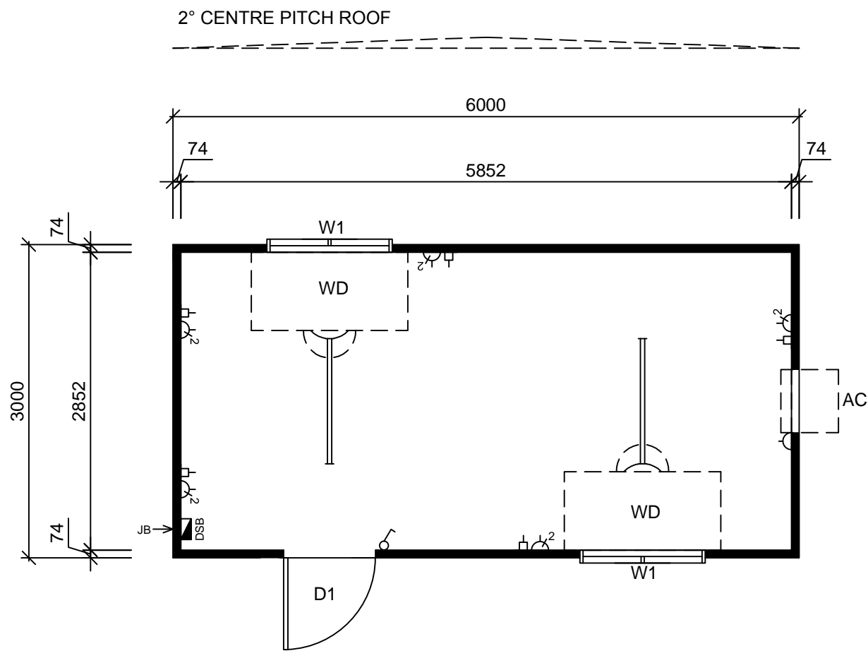
6.0x3.0m Office - Floor Plan
