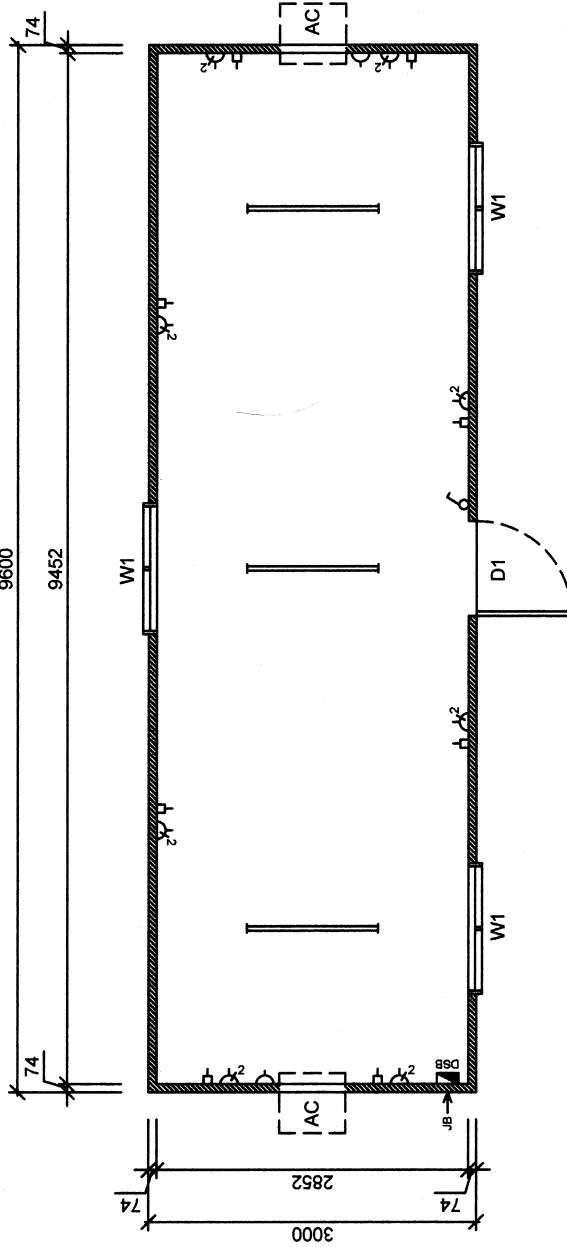
9.6x3.0m Office - Floor Plan
