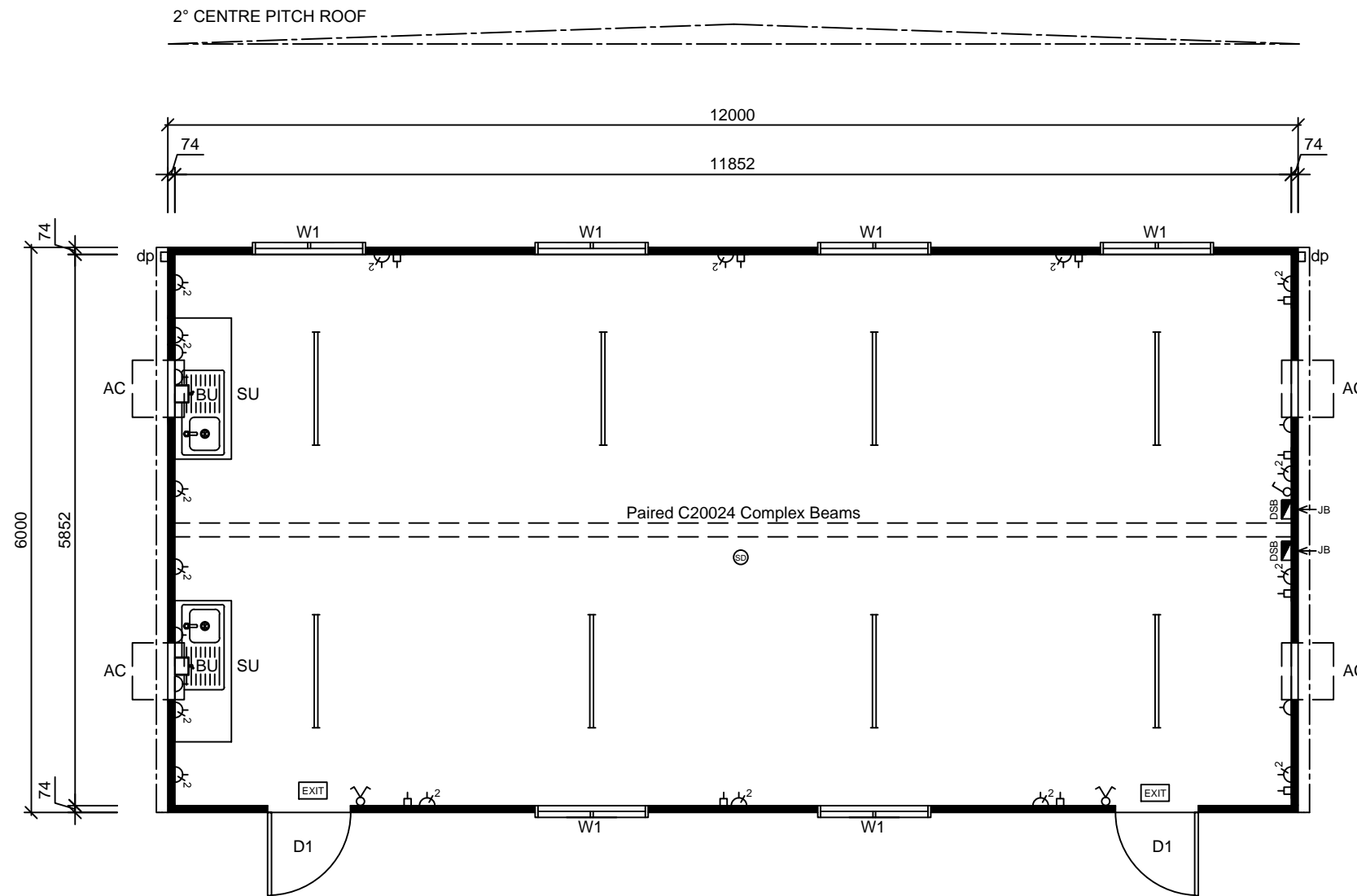
12.0x6.0m Crib Room - Floor Plan
