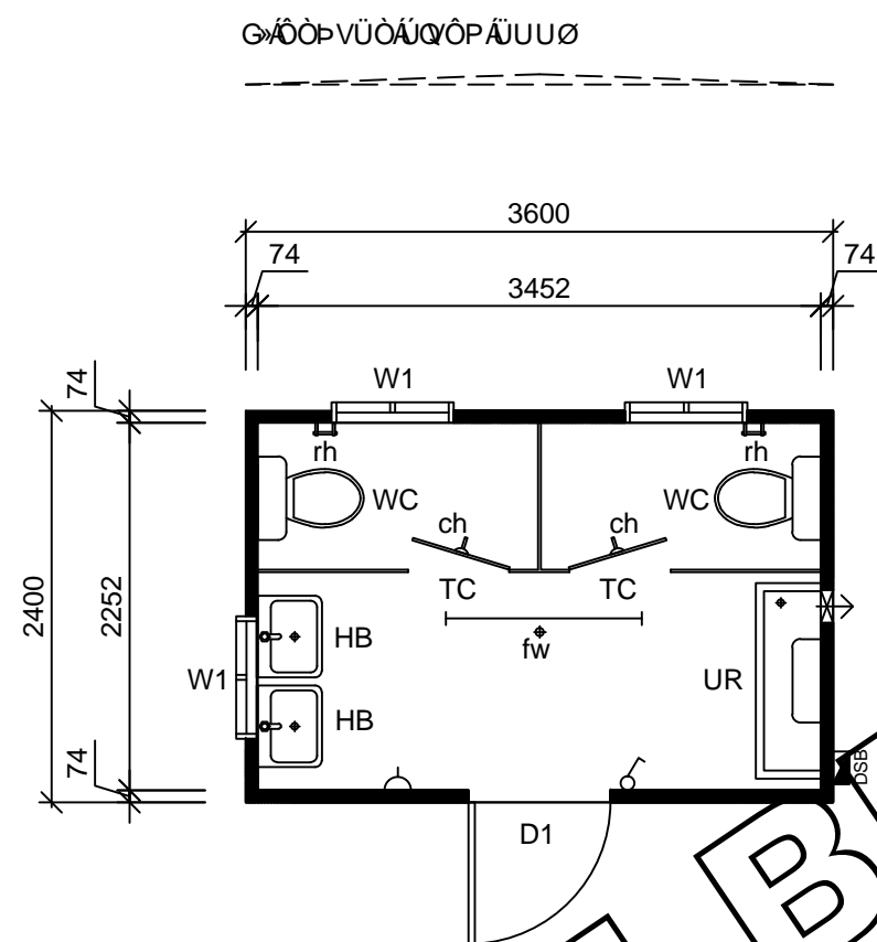
3.6x2.4m Toilet Block - Floor Plan Scale 1:50
