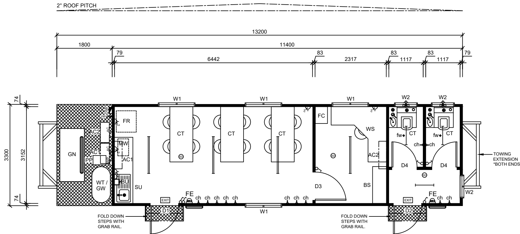
13.2x3.3m Site Building - Floor Plan
