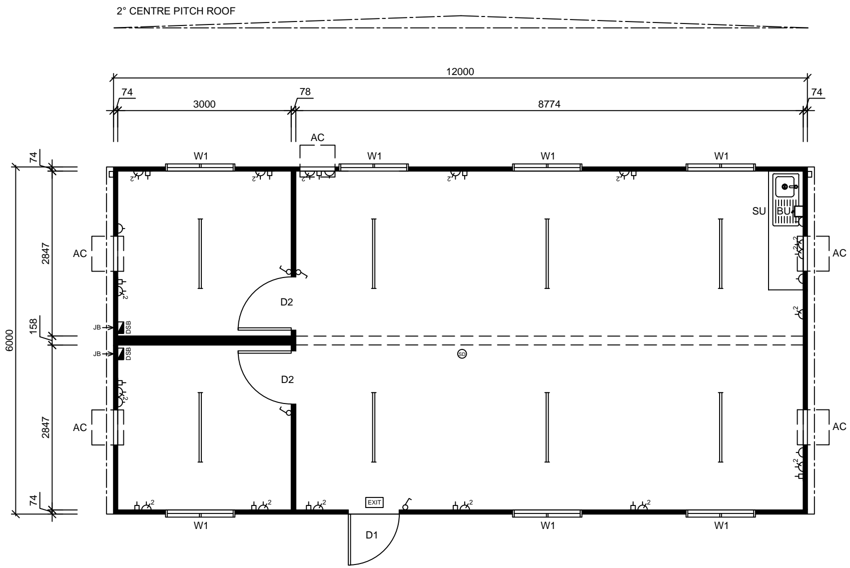
12.0x6.0m Office Complex - Floor Plan Scale 1:75
